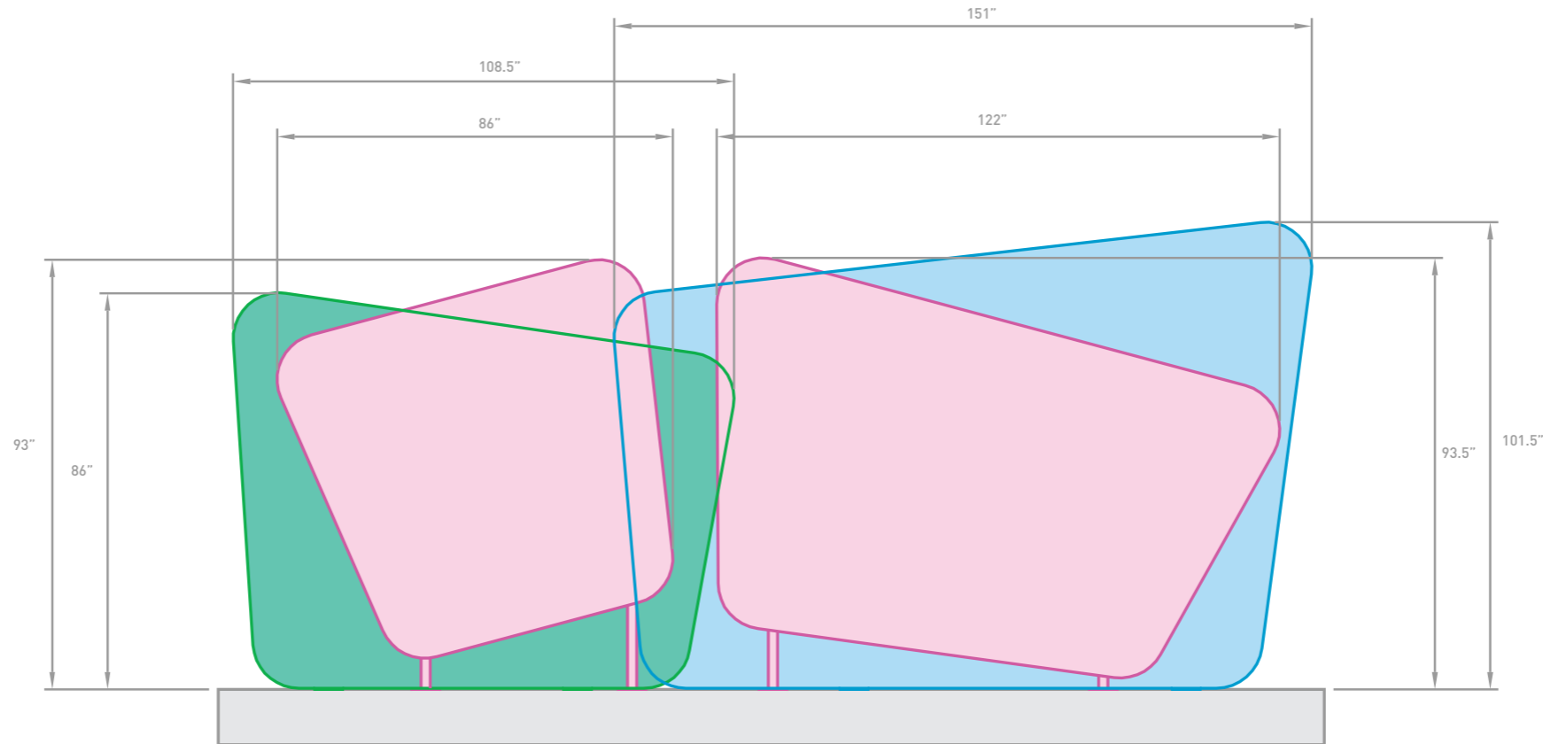
Front View
